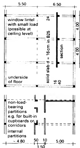
2 Structural system: multi-span beams
